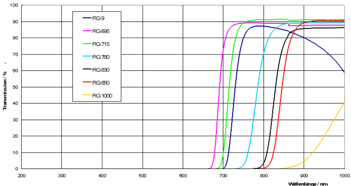
RG - Filter, Dicke 3 mm
