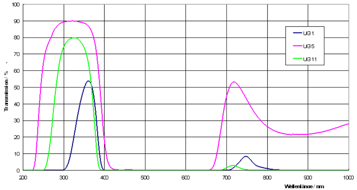
UG-Filter, Dicke 3 nm
