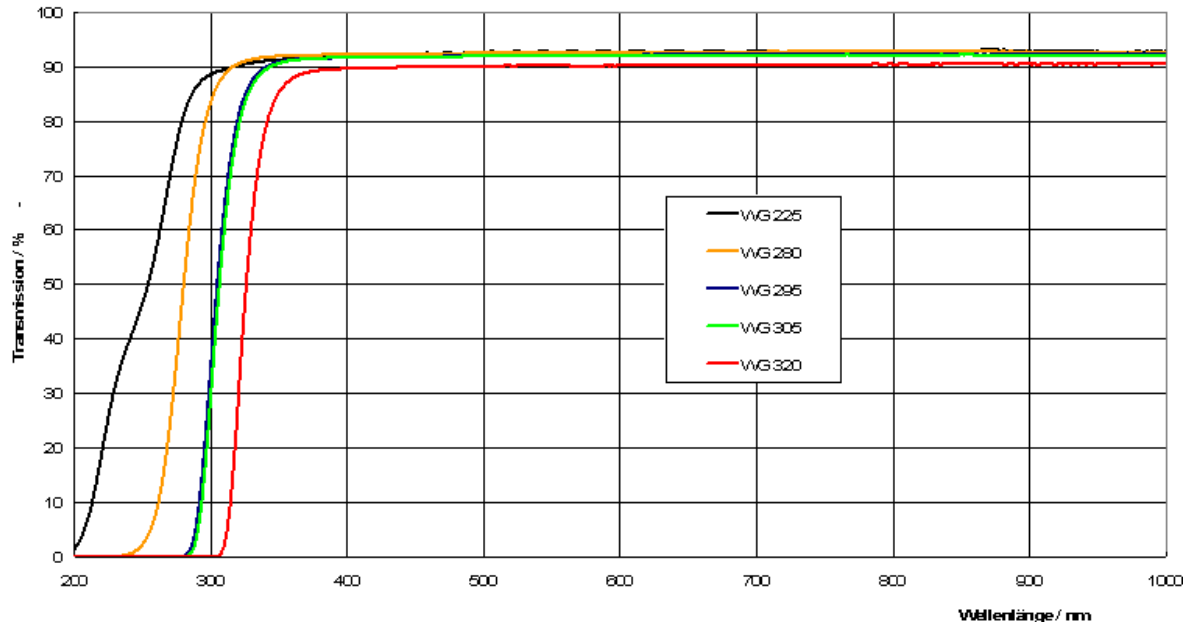
WG - Filter, Dicke 3mm
