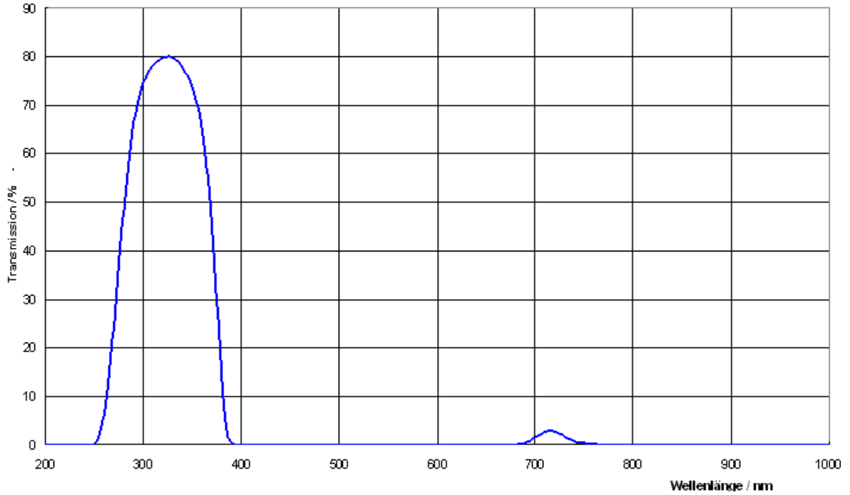
UG 11, Dicke 3 mm
